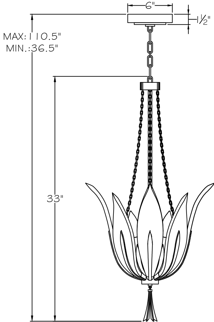
FRONT VIEW
