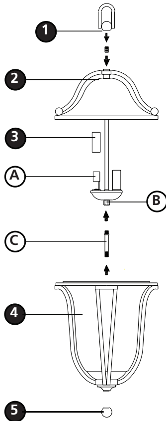
Drawing 1 - Fixture Assembly
